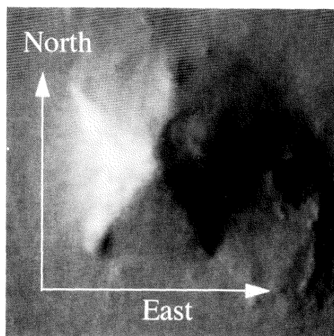
Fig. 14 D&M pyramid in 70A 13 warped to a Mercator projection.
