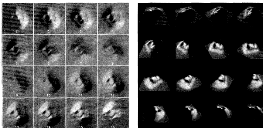
Fig. 8. Face rendered under simulated summer lighting conditions (left) and from different perspectives (right).
