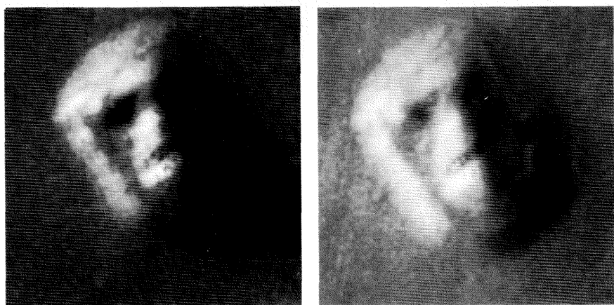
Fig. 4. Two images of the Face from 35A72 (left) and 70A13 (right).
