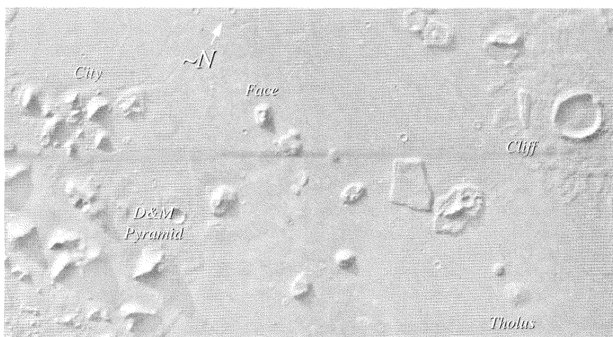
Fig 1 Mosaic of several Viking Orbiter frames from orbit 35 showing the objects under consideration on the surface of Mars. The image covers an area roughly 70 x 40 km in size. The Face, near the center of the picture, is located at approximately at 41° N latitude and 9.5° E longitude
