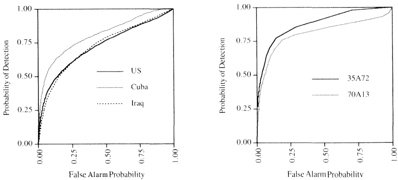
Fig. A-2. ROC curves for fractal technique for three terrestrial scenes (left) and two images containing Face on Mars (right)
