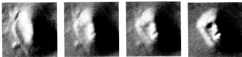
Fig. 10. Sequence fading from rounded formation (left) to the Face (right) These images from 35A72 have not been rotated or scaled in size
