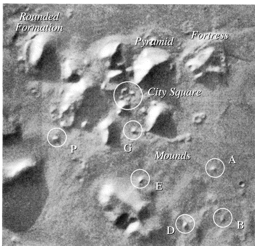
Fig. 2 The City is a collection of formations located about 30 km southwest of the Face originally identified by Hoagland. Three objects comparable in size to the Face and a number of smaller mound-like objects shown above (front 35A72) are considered here.
