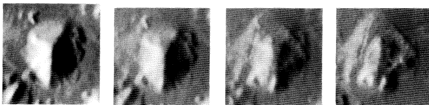
Fig. 12. Sequence derived from coregistered images from 70A11 and fade from pyramid (left) to Fortress (right). The images have not been rotated or scaled in size.
