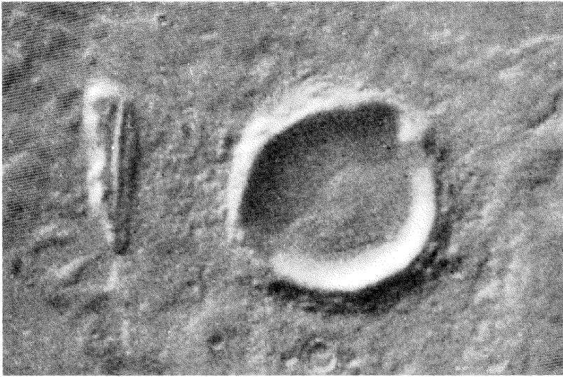
Fig. 16. Cliff and adjacent impact crater.
