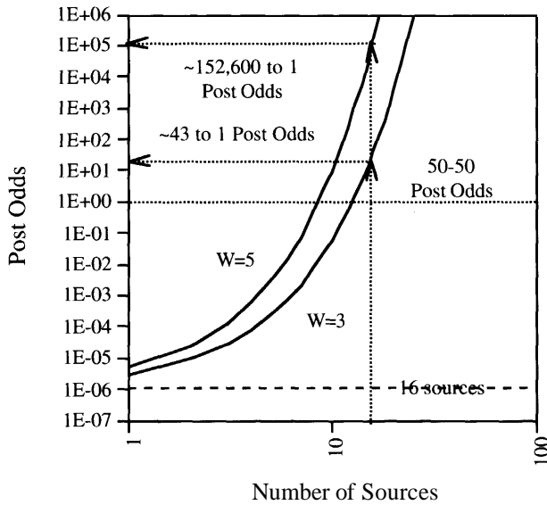
Figure 18. Post odds for N=16 sources with individual source likelihood ratios between 3 and 5.
