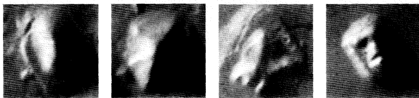
Fig. 11. Similarity in orientation and scale of four objects (from 35A72). As in previous figures, these images have not been rotated or scaled in size
