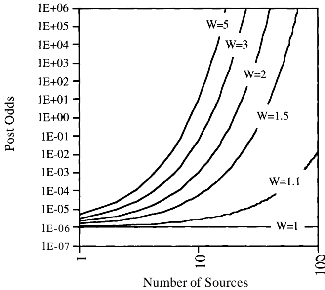
Fig. 17. Post-odds increases dramatically as the number of sources increases for weights greater than one.
