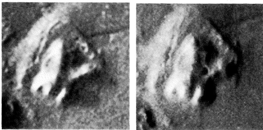
Fig. 11 Two images of fortress from 35A72 (left) and 70A11 (right)
