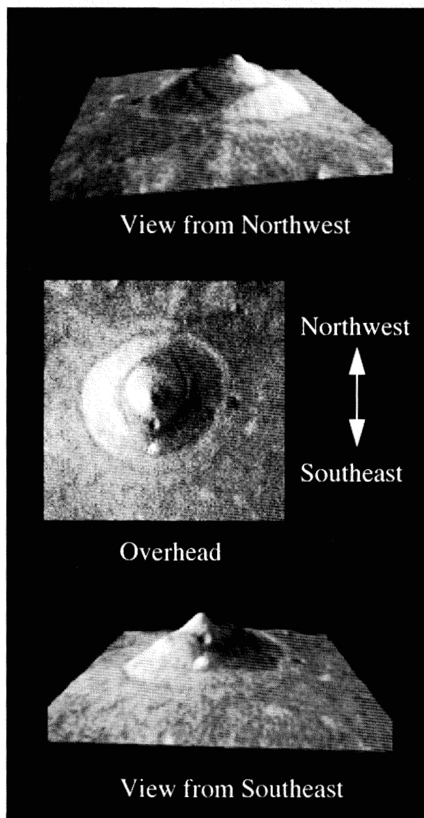
Fig. 15. Overhead view of Tholus from 35A74 along with two perspective views generated from the overhead image using shape from shading and image perspective transformation.
