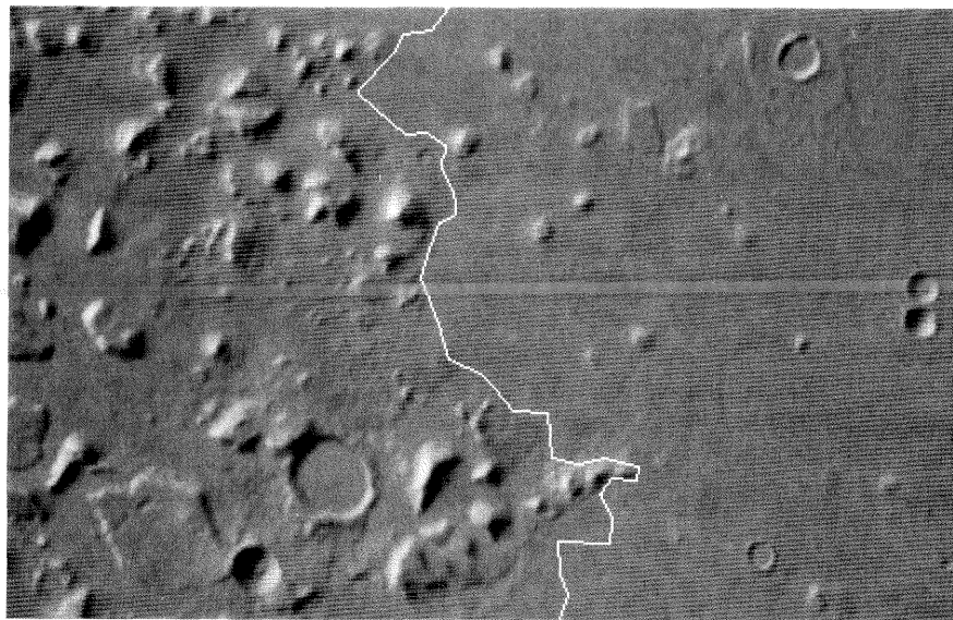
Fig. 3. Boundary between knobby terrain (left) and cratered terrain (right). Face and City at top middle.
