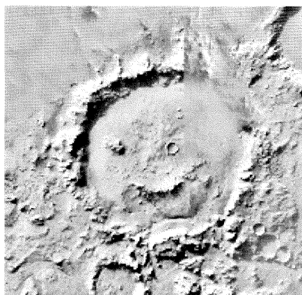
Fig. 5. Crater with internal features resembling a 'Smiley Face' used to illustrate human tendency to see faces in nature
