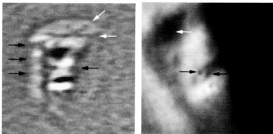
Fig. 7. Subtle details in Face. Contrast enhanced image left showing broad stripes (black arrows) and crossed lines (white arrows). Magnified image on right shows eyeball (white arrow) and "teeth" (black arrows).
